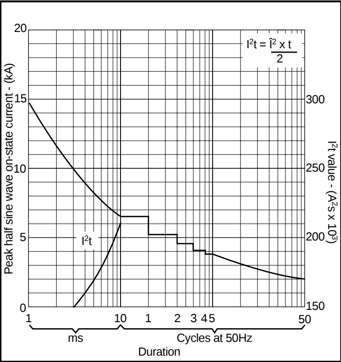
Fig. 4 Surge (non-repetitive) on-state current vs time (with 50% V_{\text{RSM}} at T_{\text{case}} = 125^\circ\text{C} )
