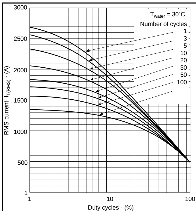
Fig. 8 Single phase welding rating @ T_{\text{water}} = 30^{\circ}\text{C}
