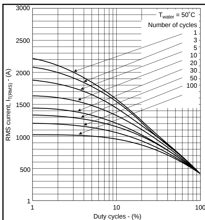
Fig. 10 Single phase welding rating @ T_{\text{water}} = 50^{\circ}\text{C}
