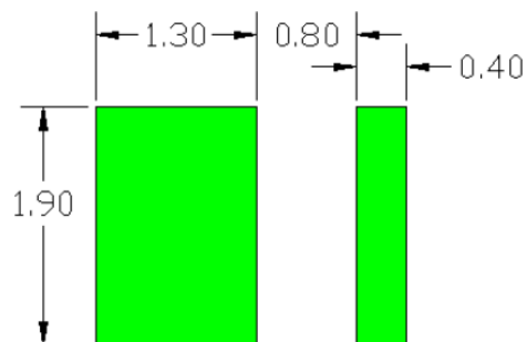
Recommended stencil opening
