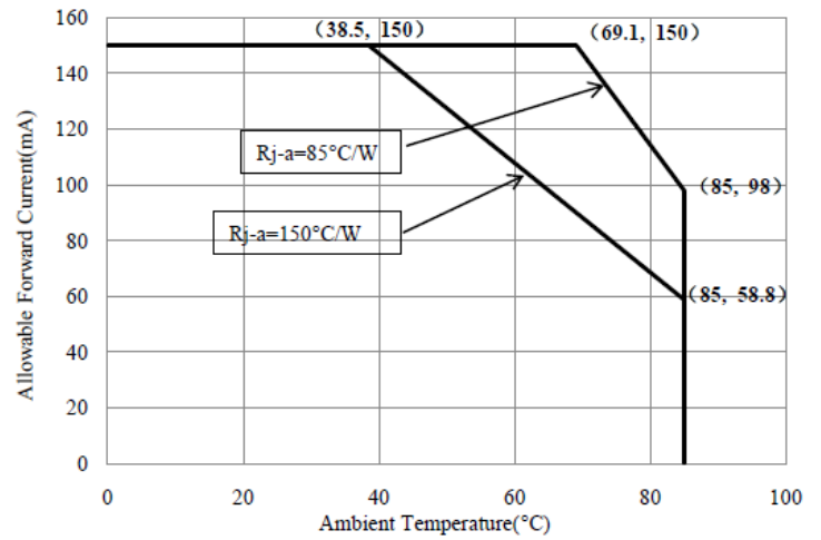
Ambient Temperature-Allowable Forward Current
