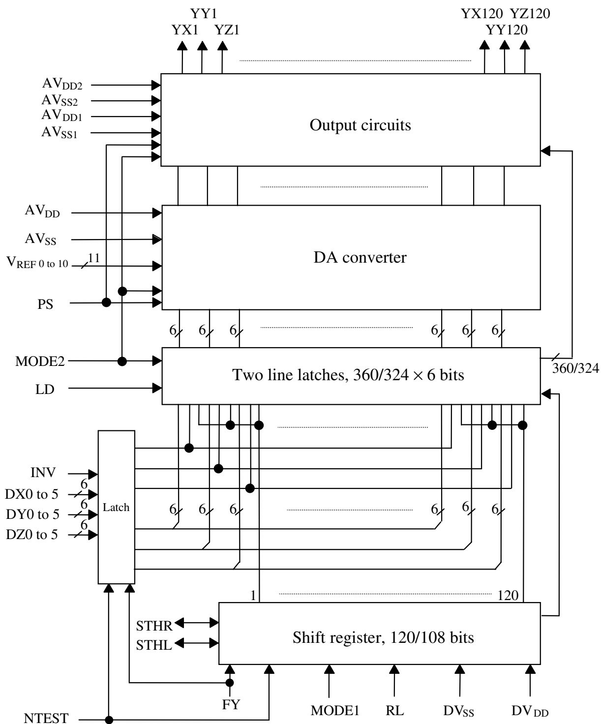
Figure 4.1 Block Diagram
