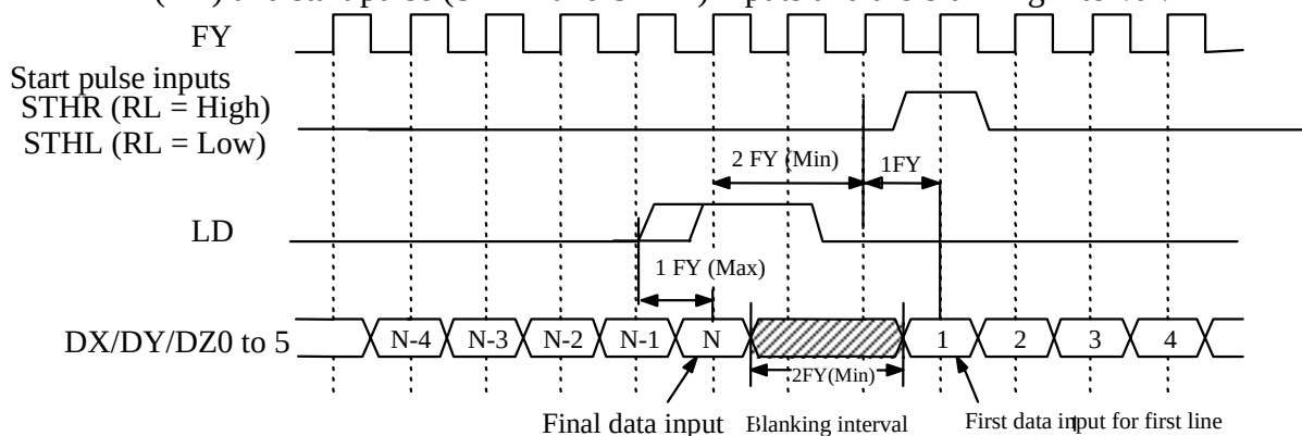
Figure 6.4 Blanking Interval
