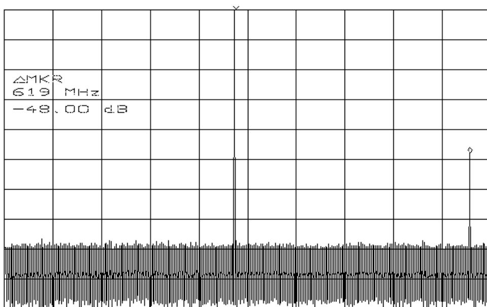
MN725-0625.0000 Output Spectrum from 1 MHz to 1.3 GHz
