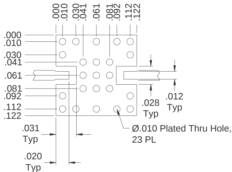
QFN-Package Doubler Surface-Mount Landing Pattern
