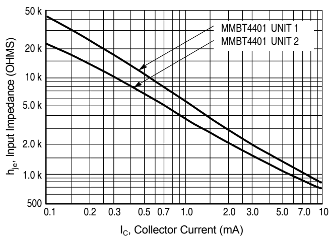
Figure 12. Input Impedance
