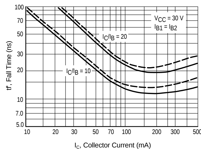
Figure 8. Fall Time
