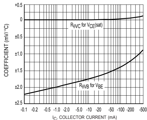
Figure 10. Temperature Coefficients
