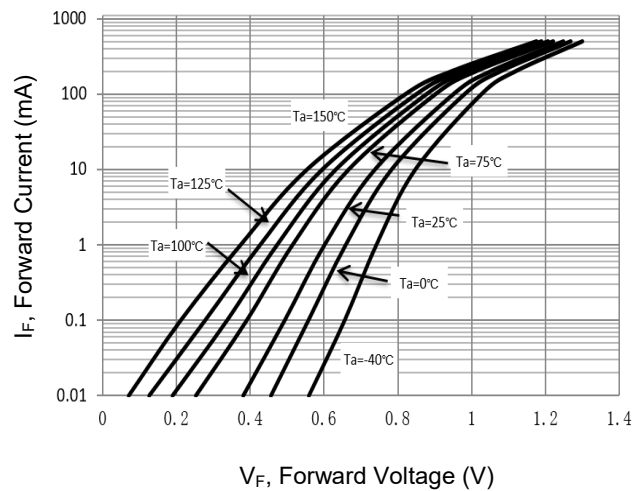
Fig 4. Forward Characteristics
