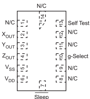
Figure 4. Pinout Description
