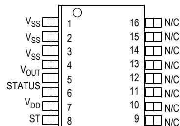
Figure 2. Pin Connections
