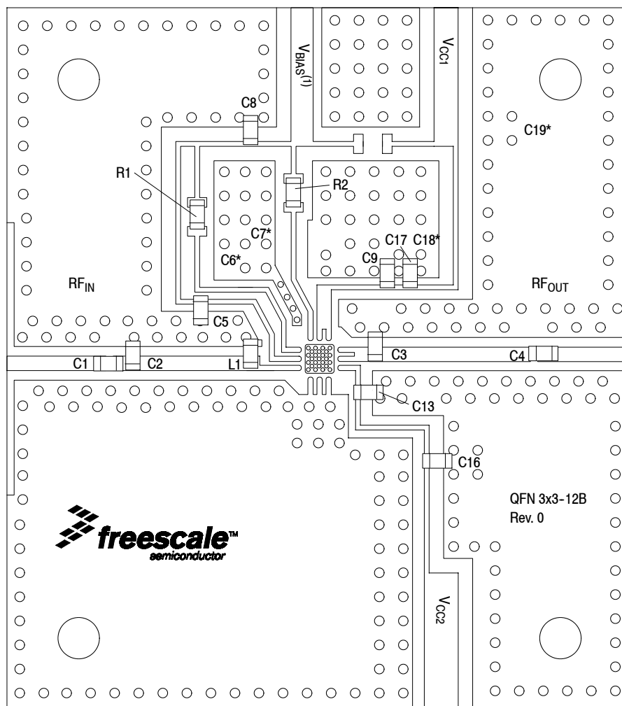
(1) V_{BIAS} [Board] supplies V_{BA1} , V_{BA2} and V_{BIAS} [Device]. Note: Component numbers C6*, C7*, C18* and C19* are labeled on board but not placed.
