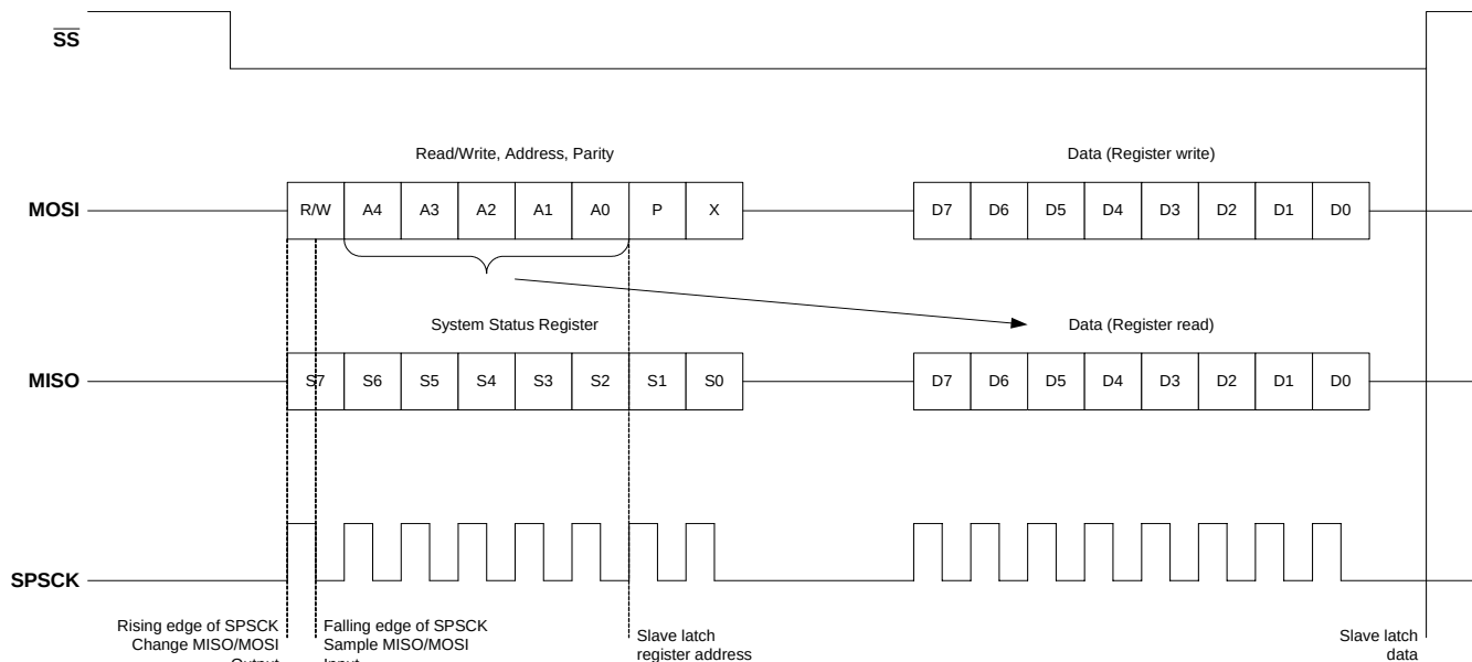
Figure 29. SPI Protocol
