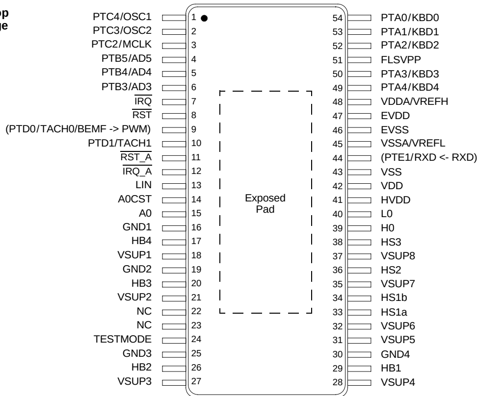
Figure 3. Terminal Connections
