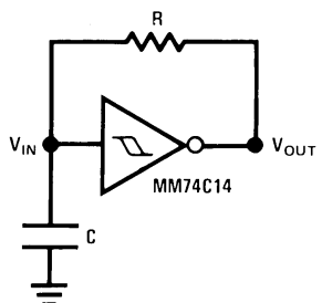
Low Power Oscillator
