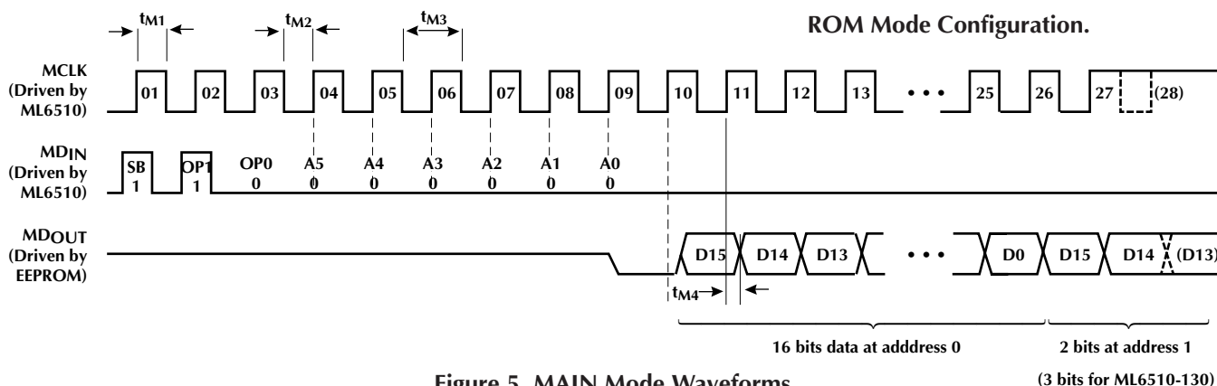
Figure 5. MAIN Mode Waveforms.
