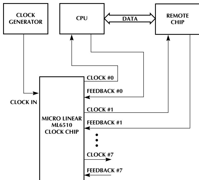
Figure 1. Basic System Configuration Using the ML6510.
