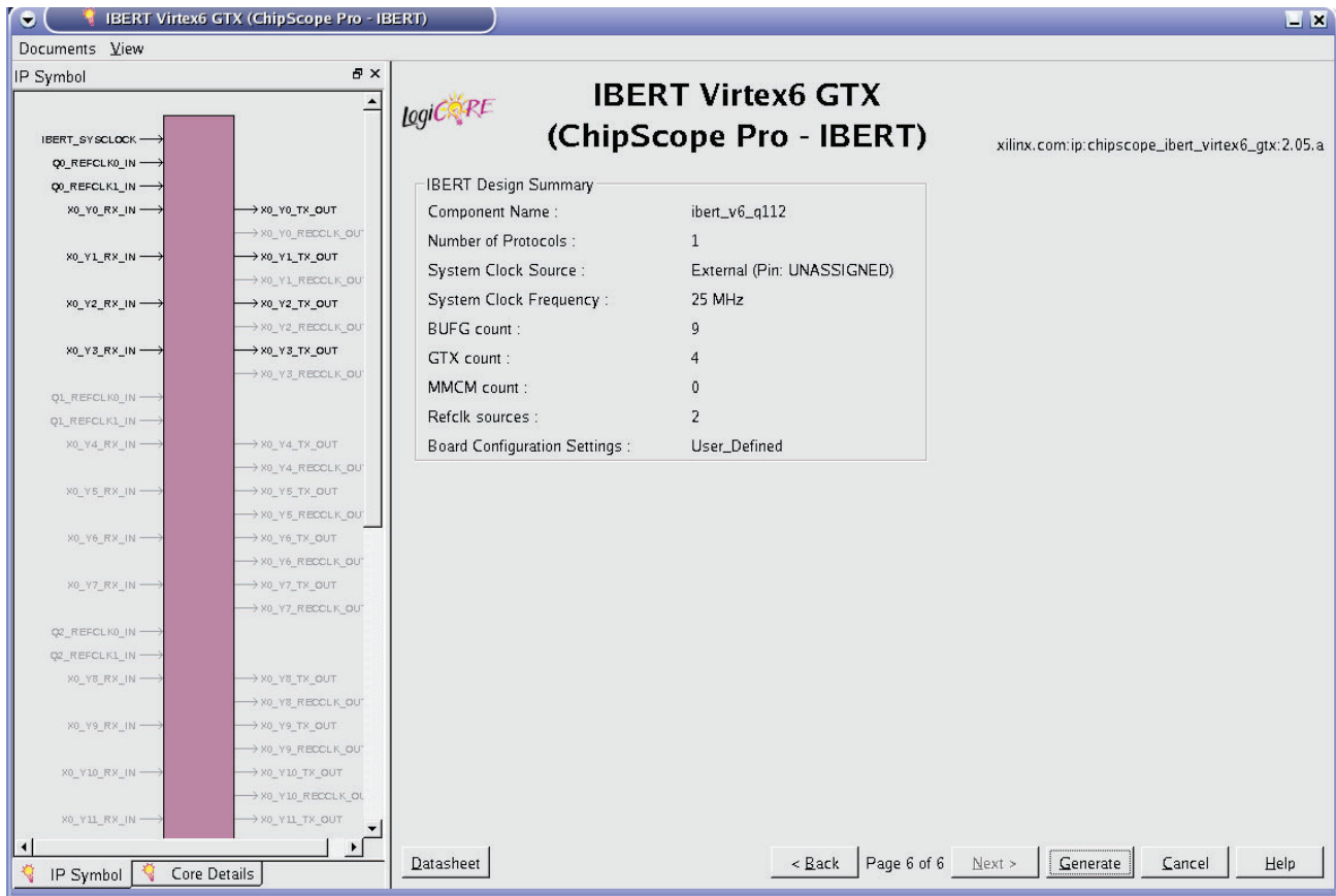
Figure 1-30: IBERT Design Summary
