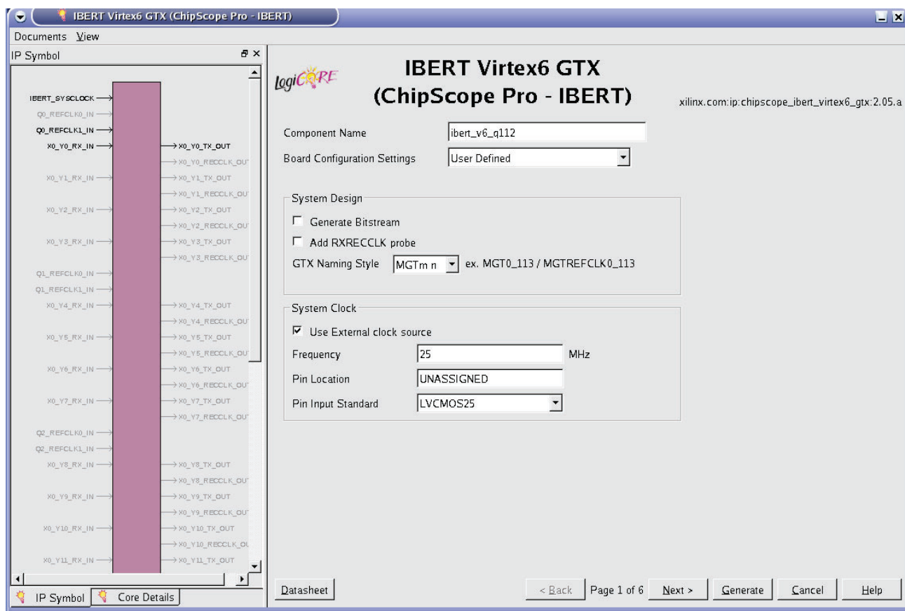
Figure 1-25: IP Customization, Page 1
