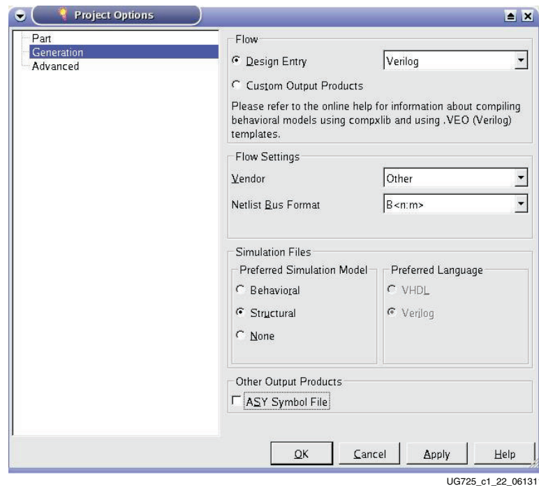
Figure 1-22: Generation Options
