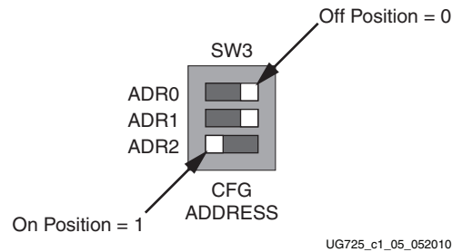
Figure 1-5: Configuration Address DIP Switch (SW3)
