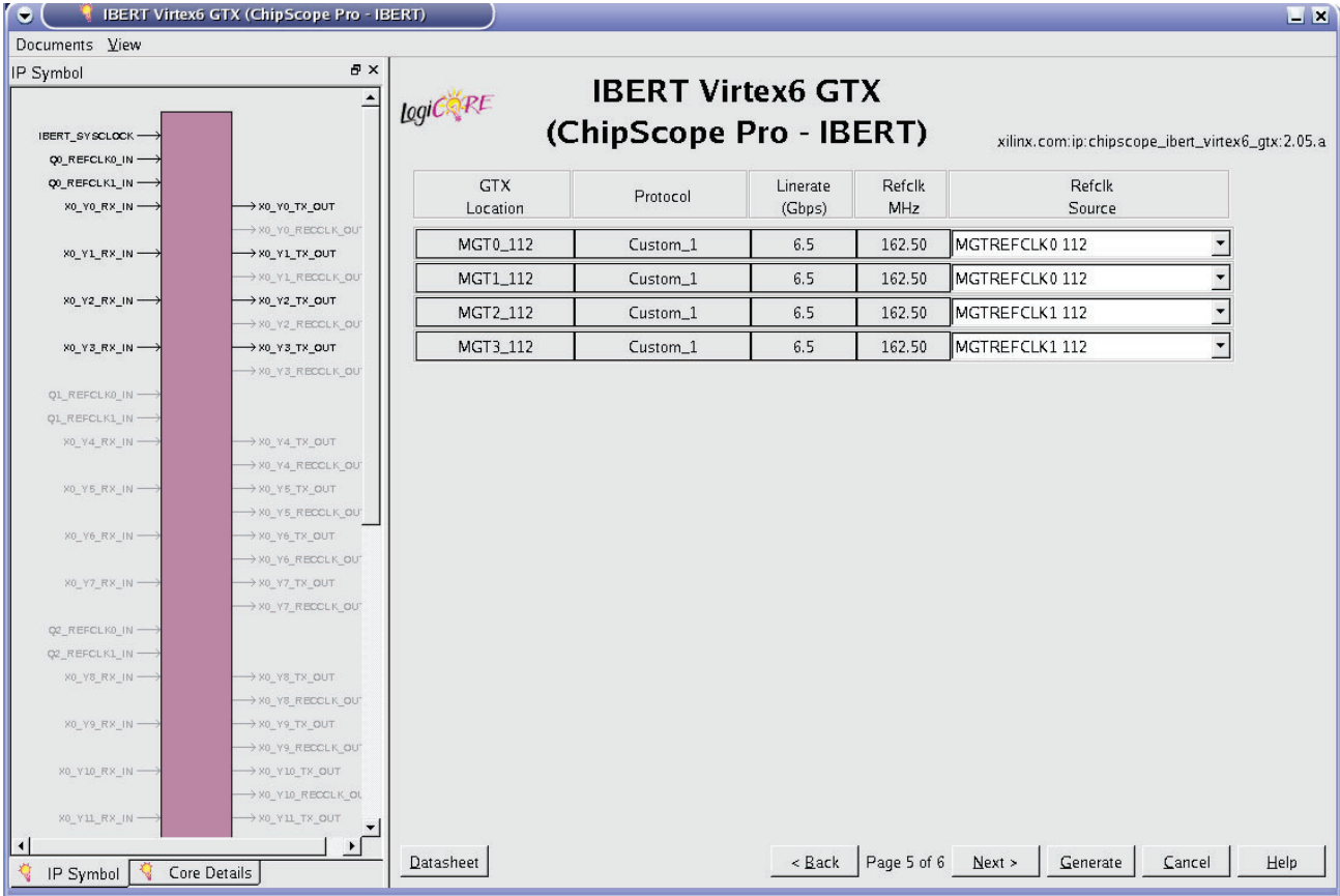
Figure 1-29: IP Customization, Page 5
