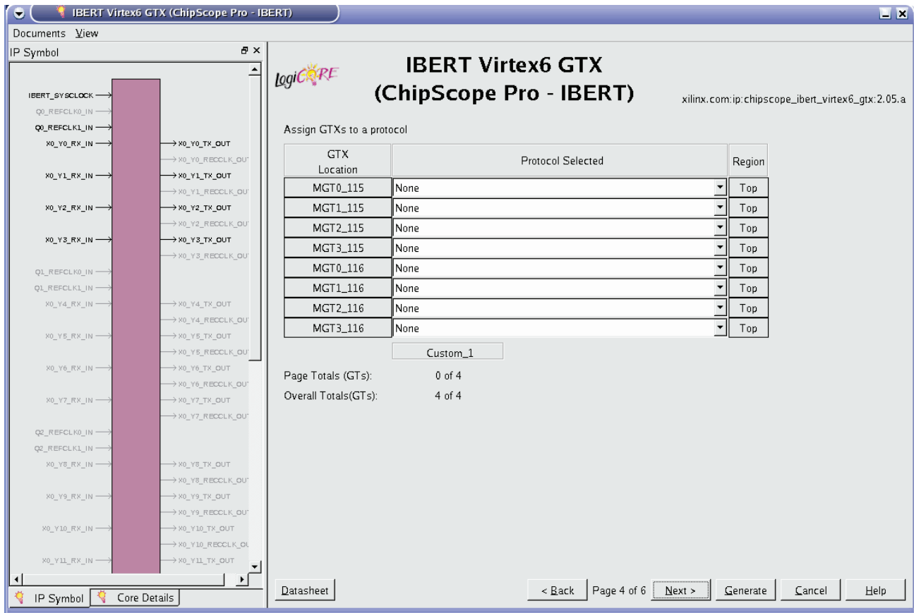
Figure 1-28: IP Customization, Page 4
