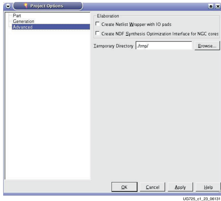
Figure 1-23: Advanced Options
