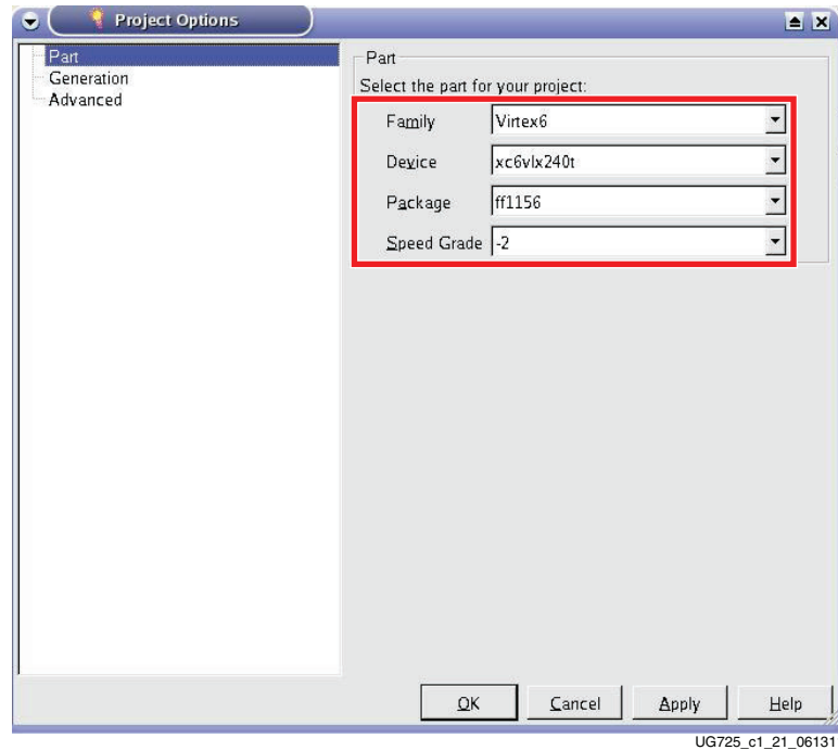
Figure 1-21: Part Options
