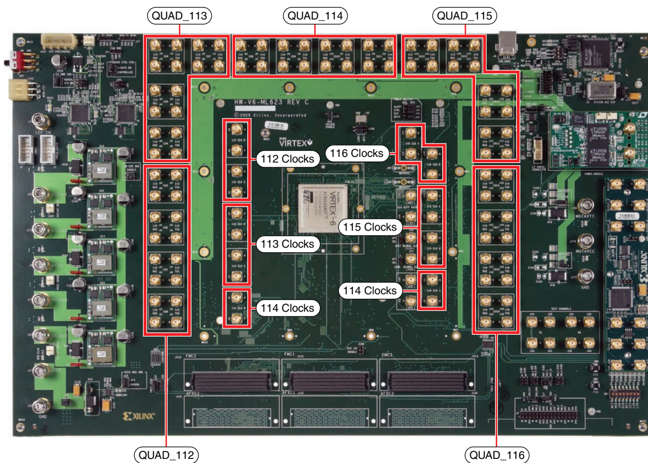
Figure 1-7: GTX Transceiver and Reference Clock SMA Locations
