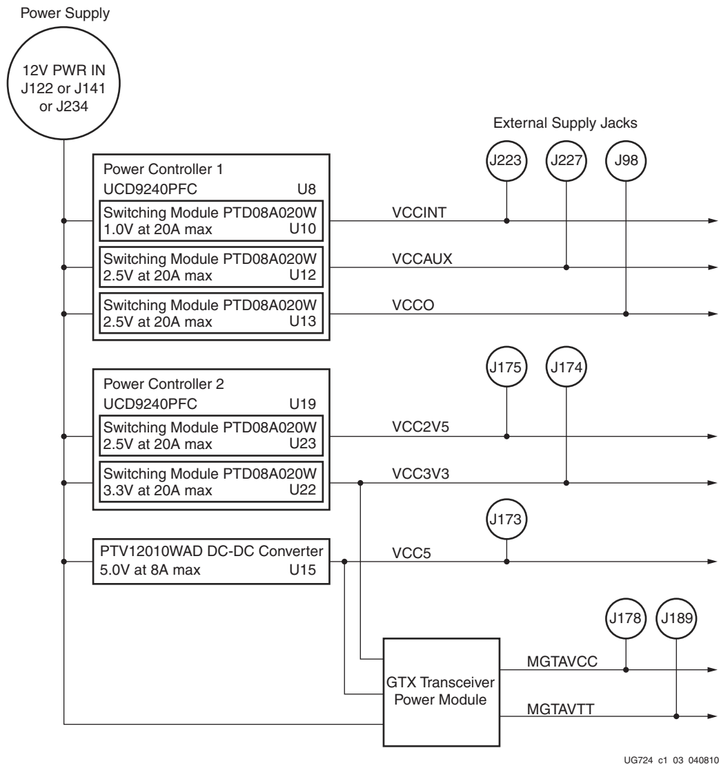
Figure 1-3: ML623 Board Power Supply Block Diagram
