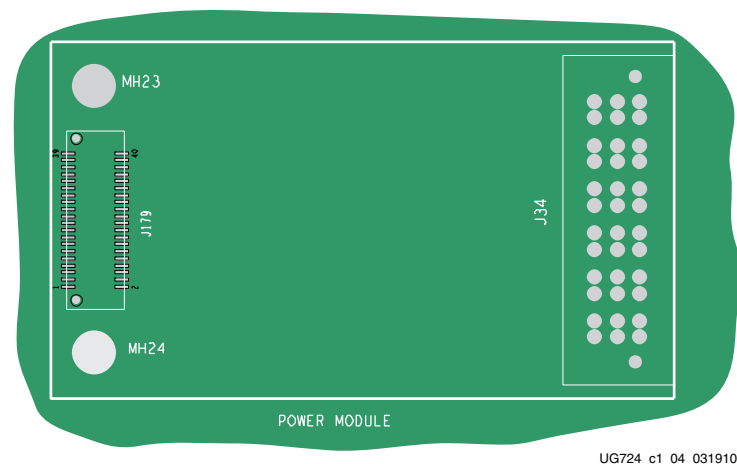
Figure 1-4: Mounting Location, GTX Transceiver Power Module
