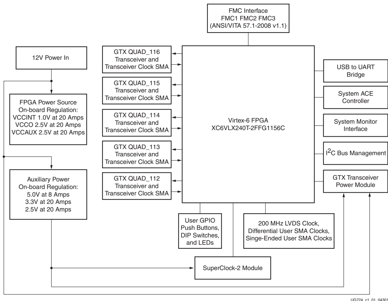
Figure 1-1: ML623 Board Block Diagram
