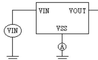
Test Circuit 2
