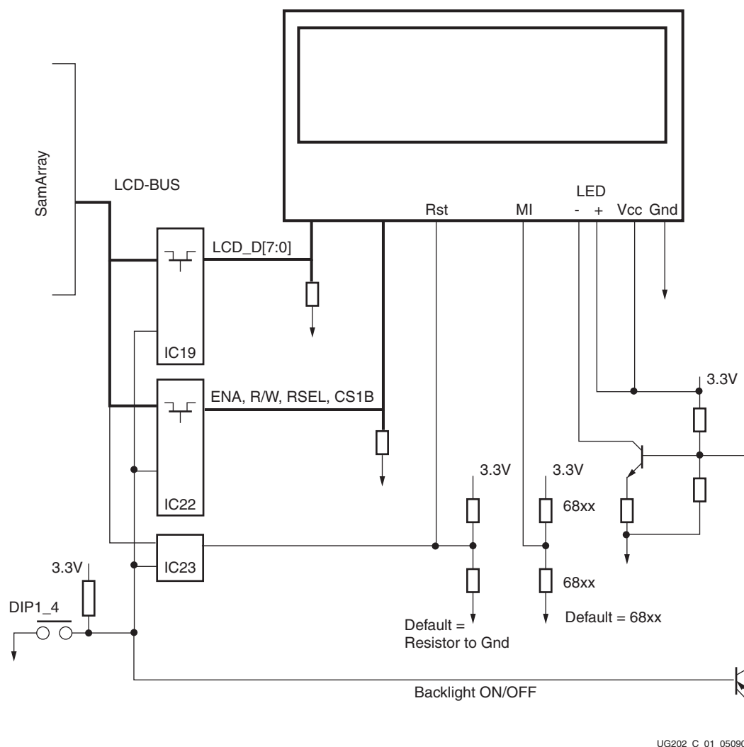
Figure C-1: Display Schematic Diagram
