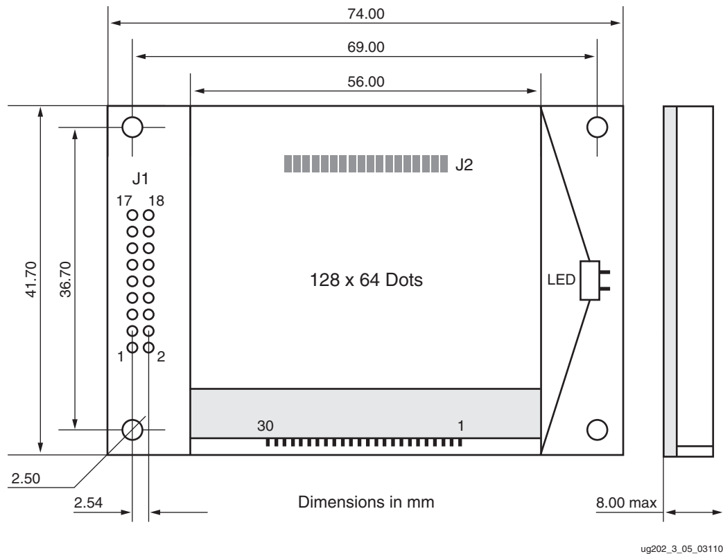
Figure 3-5: 64128EFCBC-3LP Dimensions
