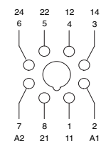
Terminal Arrangement
