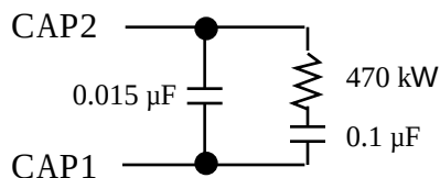
Figure 4. Loop Filter Component Values
