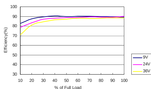
MJWI20-24S05 Efficiency vs Load Current
