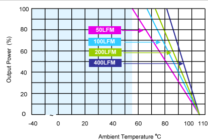
MJWI20-48S033 Derating Curve with Heatsink
