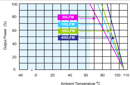
MJWI20-24S033 Derating Curve without Heatsink
