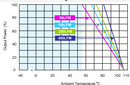
MJWI20-XXS24 Derating Curve without Heatsink
