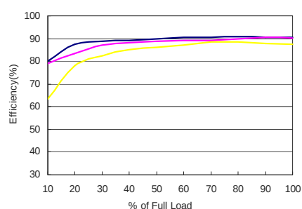
MJWI20-48S15 Efficiency vs Load Current
