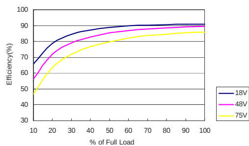
MJWI20-48S05 Efficiency vs Load Current
