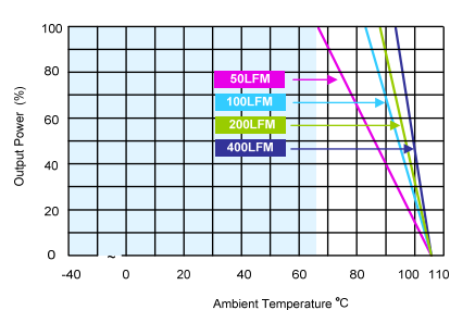
MJWI20-XXS05, MJWI20-XXS12, MJWI20-XXS15, MJWI20-XXD12, MJWI20-XXD15 Derating Curve with Heatsink
