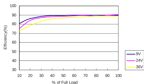
MJWI20-24S15 Efficiency vs Load Current
