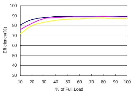
MJWI20-48S12 Efficiency vs Load Current
