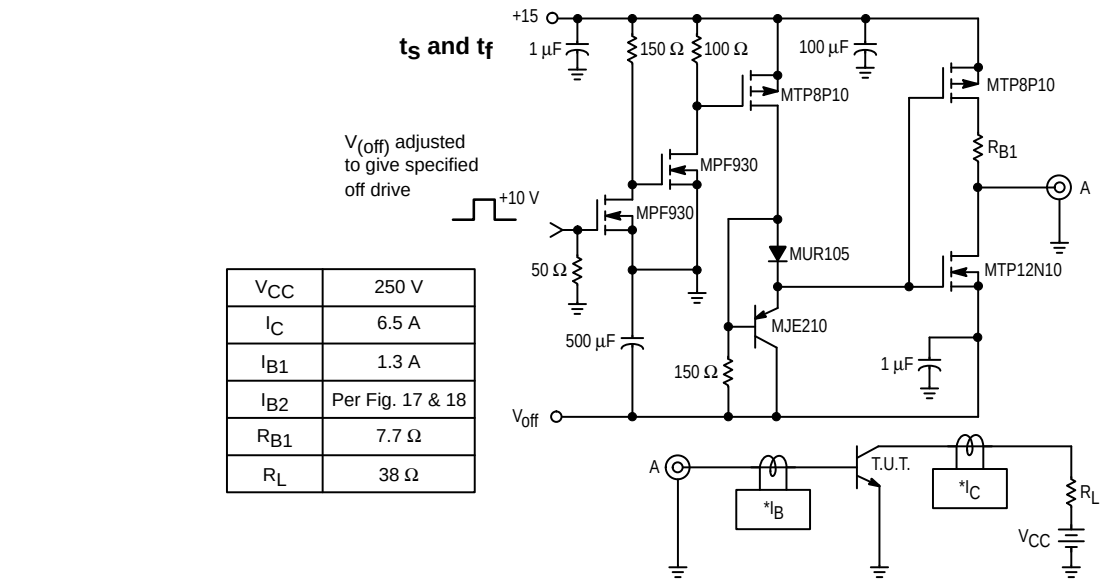
Figure 16. Resistive Load Switching
