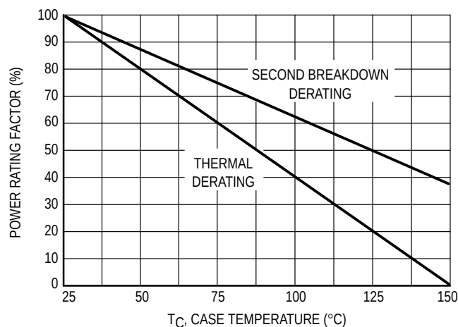
Figure 9. Power Derating
