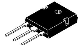
CASE 340F-02 TO-247AE
