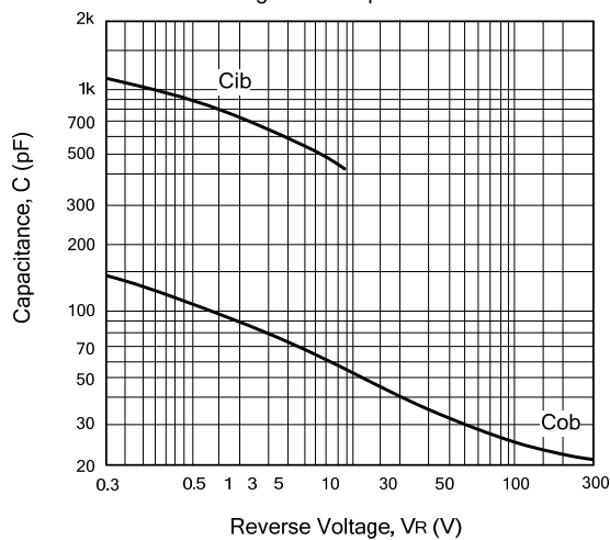
Figure 12. Capacitance
