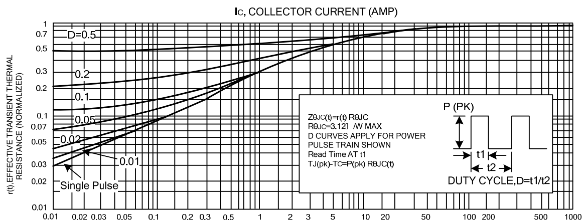
Fig 4. Thermal Response
