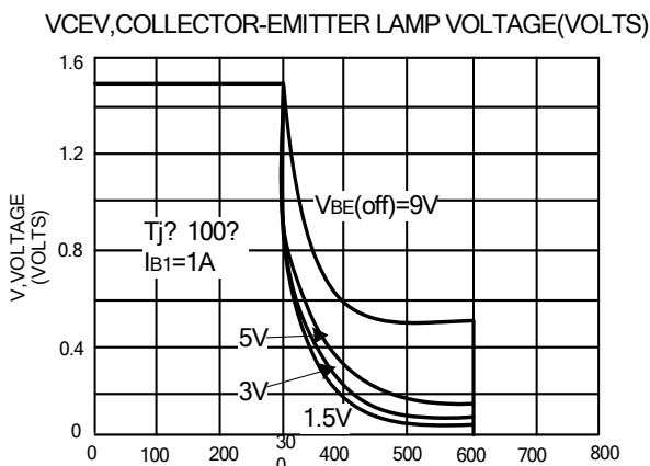
Fig 6. Reverse Bias Safe Operating Area
