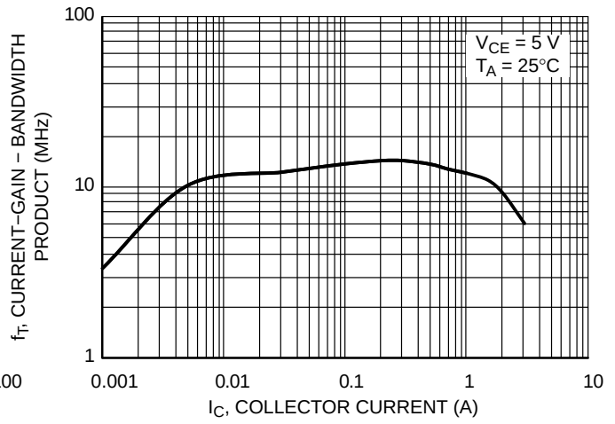
Figure 13. Current-Gain-Bandwidth Product
