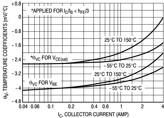
Figure 10. Temperature Coefficients
