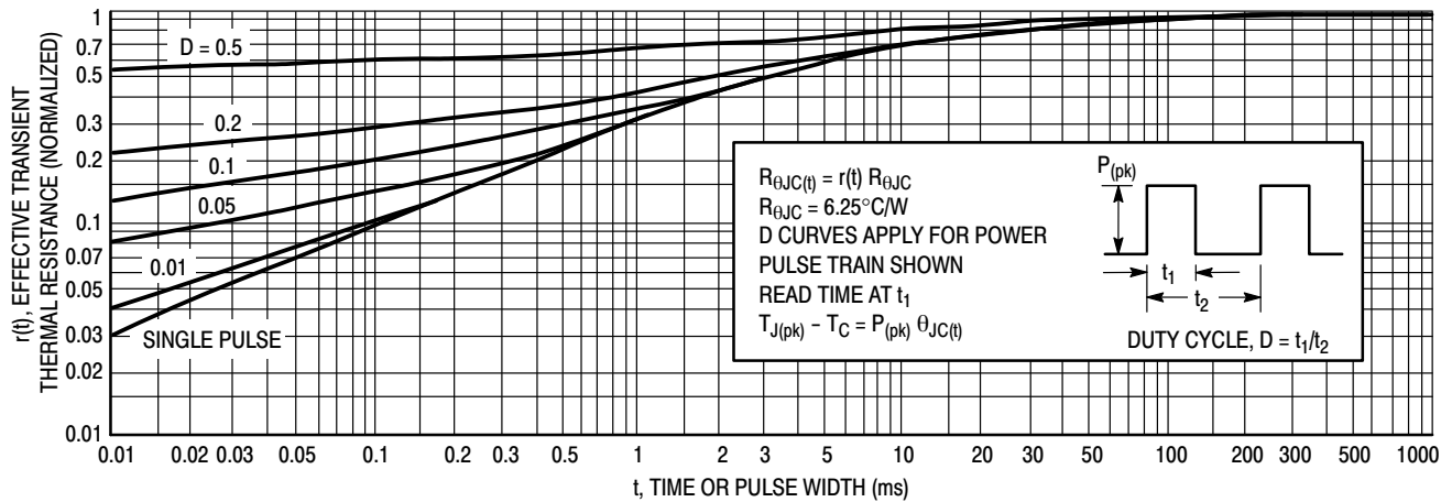
Figure 3. Thermal Response
