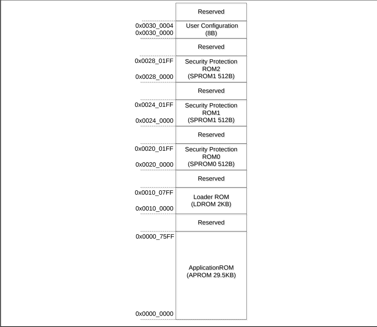
Figure 6.2-8 NuMicro® Mini57 Flash, Security and Configuration Map
