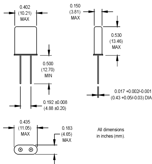
HC-49/U 00.0000 MHz (customer specified)
