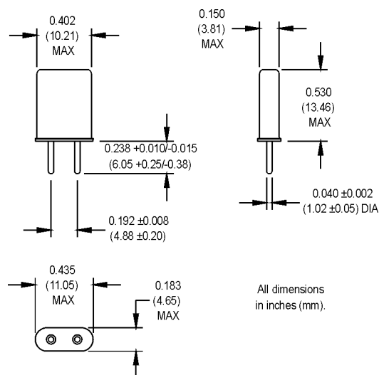
HC-50/U 00.0000 MHz (customer specified)
