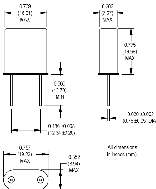
HC-51/U 00.0000 MHz (customer specified)
