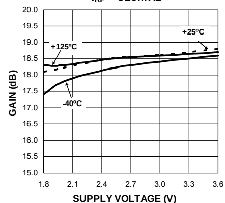
Gain vs Supply Voltage f_{RF} = 315\text{MHz}
