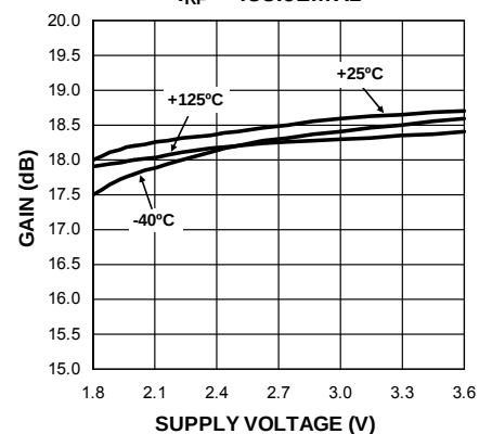
Gain vs Supply Voltage f_{RF} = 433.92\text{MHz}
