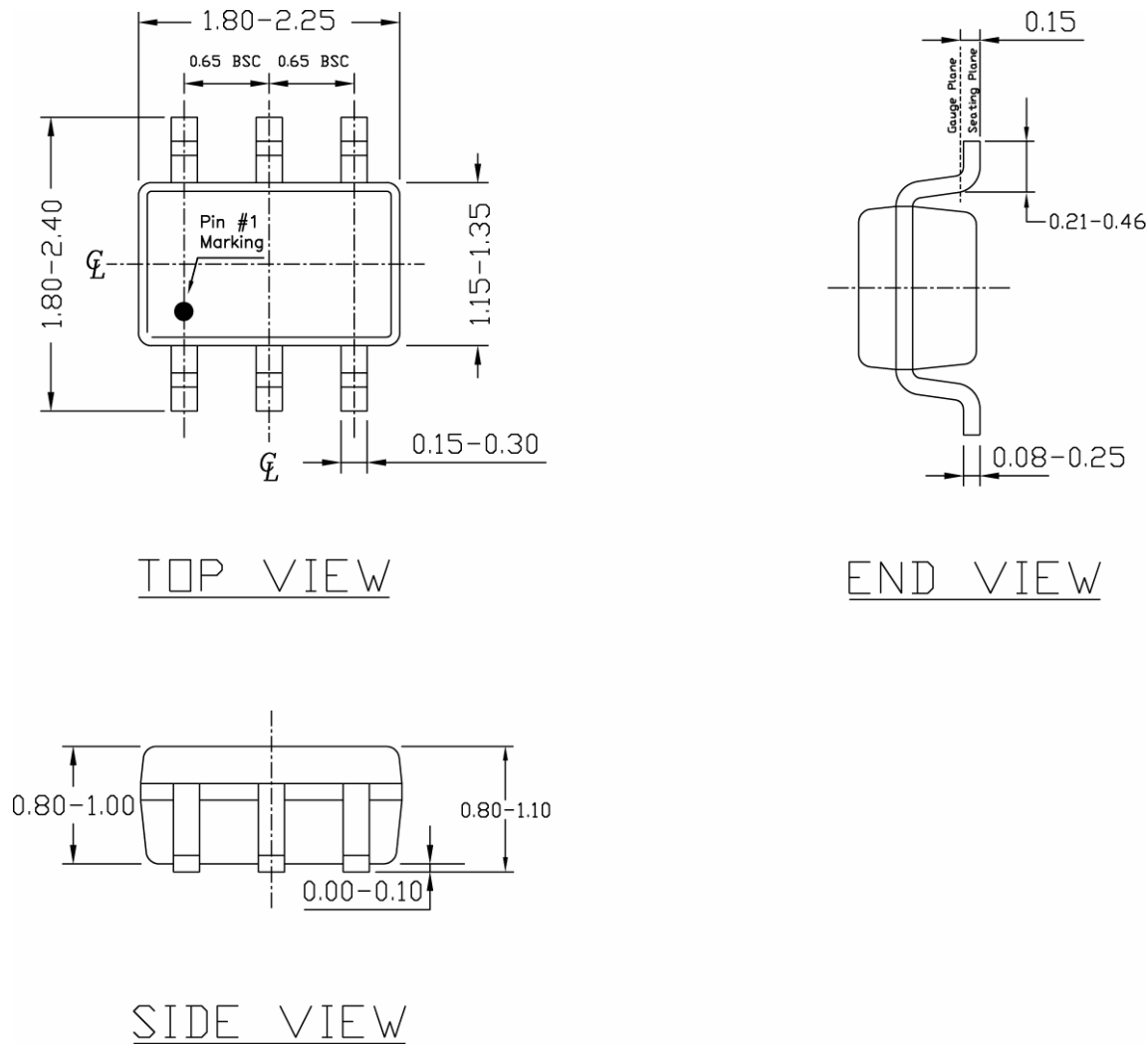
SC70-6 (C6)
