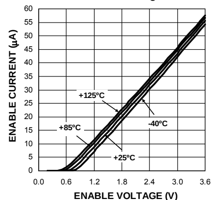
Enable Input Current vs Enable Voltage
