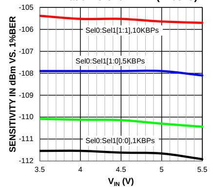
Sensitivity in 433.92MHz vs. V_{IN} at different BW in (+105°C)
