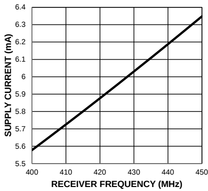
Current Vs. Receiver Frequency
