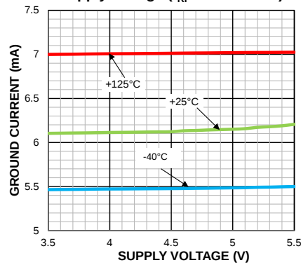
Ground Current vs. Supply Voltage ( f_{RF} = 433.92\text{ MHz} )
