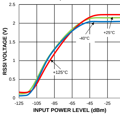
433.92 MHz RSSI Voltage vs. Input Power
