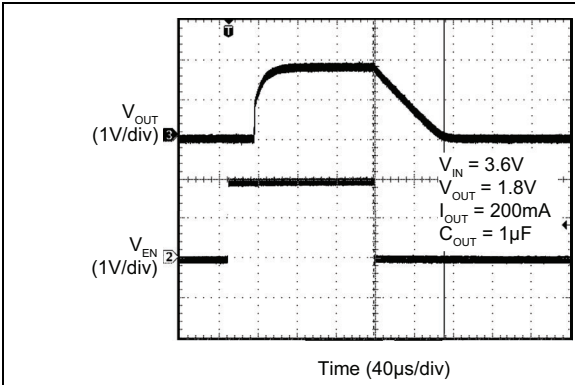
FIGURE 2-22: Enable Turn-Off.
