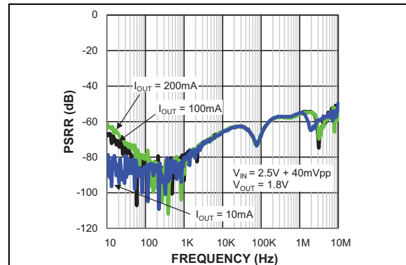
FIGURE 2-5: PSRR C_{OUT} = 2.2 \mu F .
