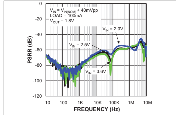
FIGURE 2-4: PSRR C_{OUT} = 1 \mu F .
