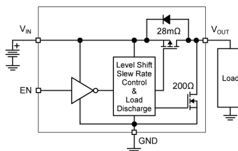
MIC94045 (1ms soft-start with auto-discharge)
