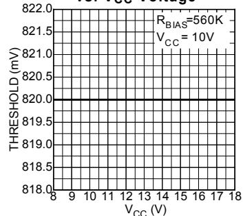
ISNS Current Limit Threshold vs. V CC Voltage
