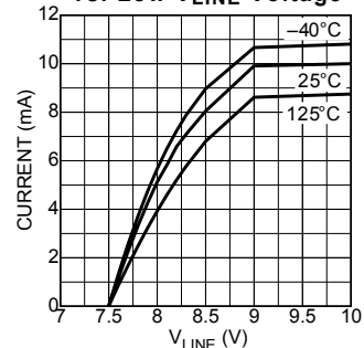
Depletion FET Current vs. Low V LINE Voltage
