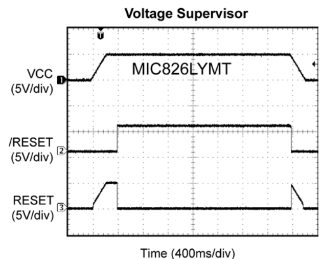
Figure 4. Voltage Supervisor Function
