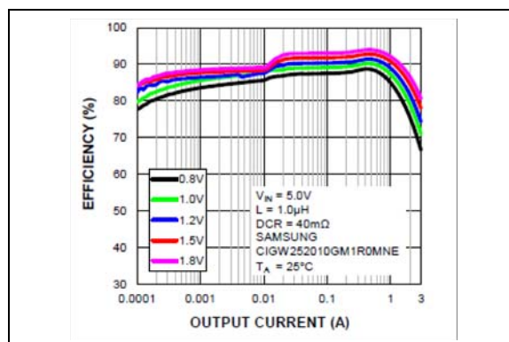
FIGURE 2-4: Buck Efficiency (LDCR = 40 mΩ) vs. Output Current.
