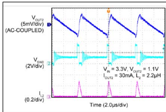
FIGURE 2-40: Buck 2 PFM Switching Waveforms.
