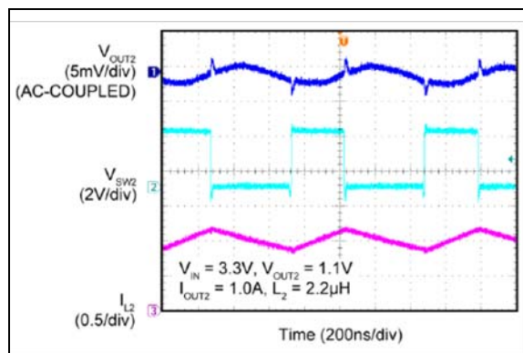
FIGURE 2-39: Buck 2 PWM Switching Waveforms.
