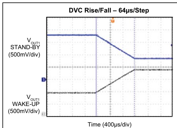
FIGURE 4-4: Buck DVC Control Ramp.
