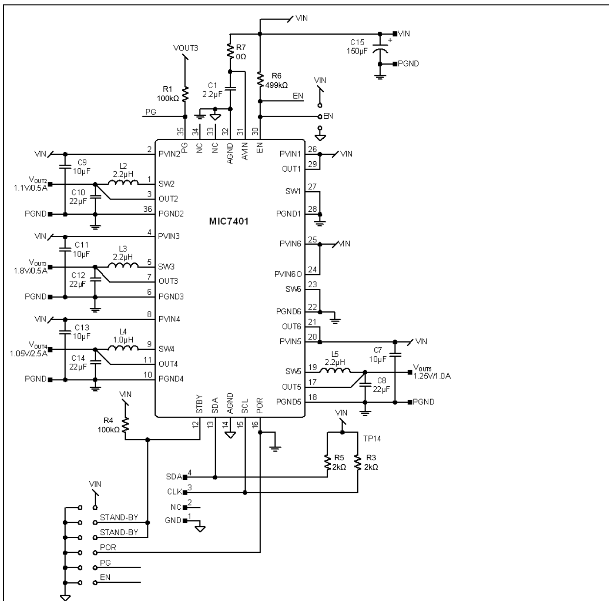
FIGURE 6-1: Connections for Unused Pins.
