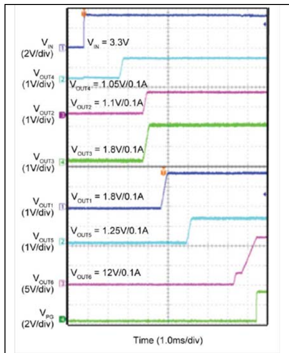
FIGURE 2-19: Hot Plug – Rising V_{IN} .
