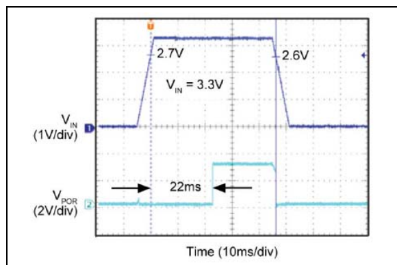
FIGURE 2-20: POR Timing.
