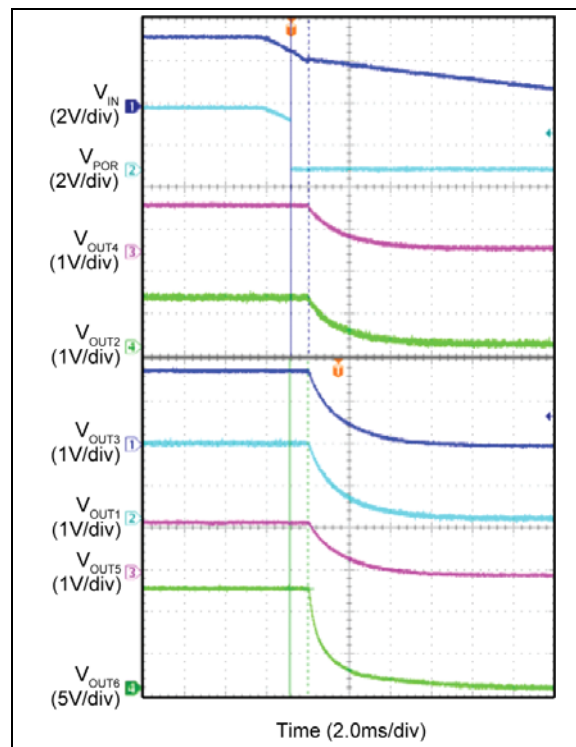
FIGURE 4-11: Hot Unplug – V_{IN} Falling.
