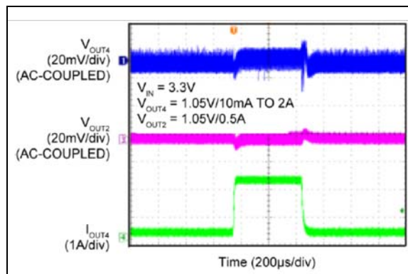
FIGURE 2-38: Cross Regulation.
