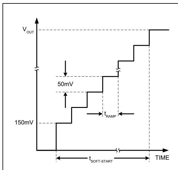
FIGURE 4-1: Buck Soft-Start.
