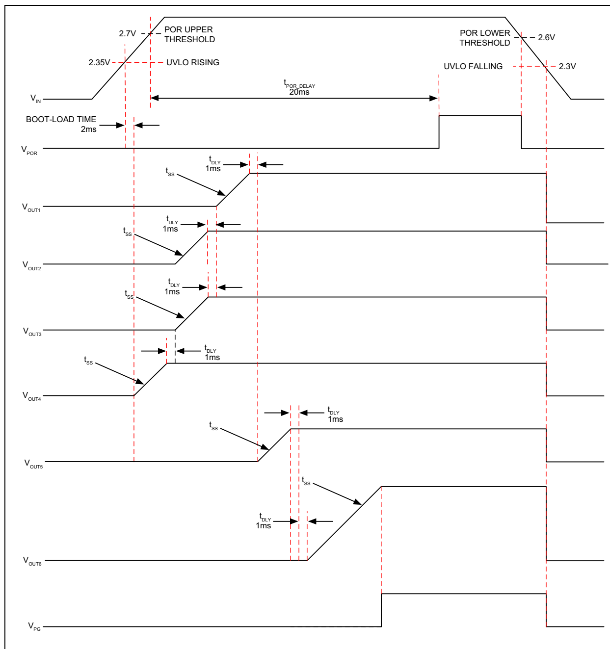
FIGURE 5-1: MIC7401 Power-Up/Down.
