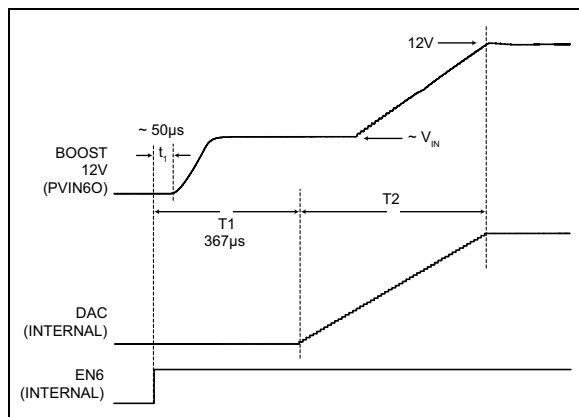
FIGURE 4-5: Boost Soft-Start Ramp.
