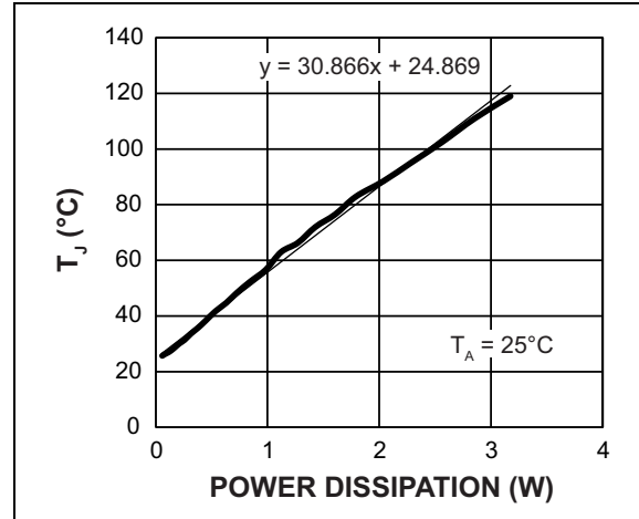
FIGURE 4-16: Power Dissipation.
