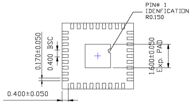
BOTTOM VIEW
