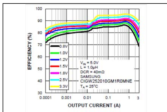
FIGURE 2-5: Buck Efficiency (LDCR = 40 mΩ) vs. Output Current.
