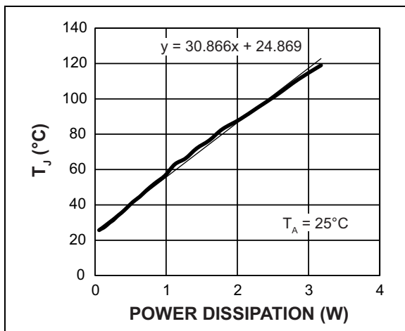
FIGURE 4-16: Power Dissipation.
