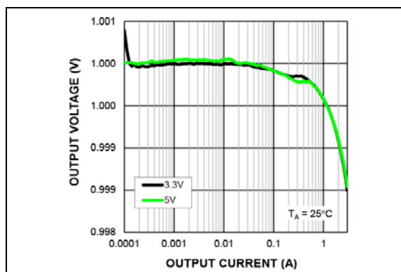
FIGURE 2-10: Buck Output Voltage (1.0V) vs. Output Current.
