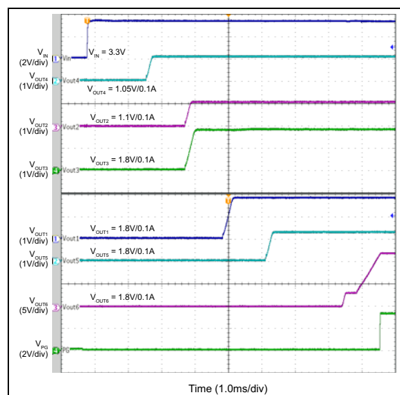
FIGURE 4-9: Hot Plug – V_{IN} Rising.
