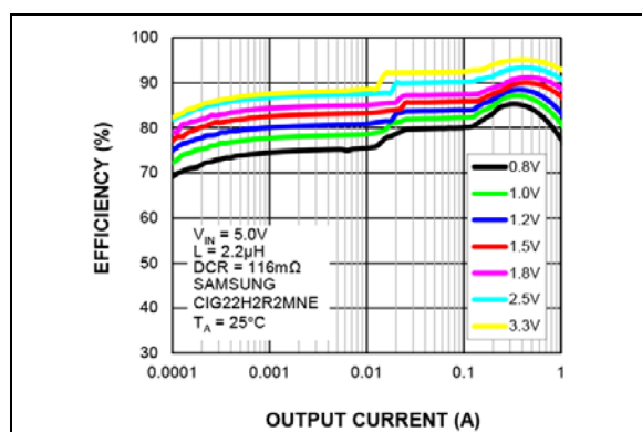
FIGURE 2-8: Buck Efficiency (LDCR = 116 mΩ) vs. Output Current.
