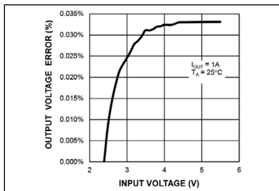
FIGURE 2-12: Buck Line Regulation vs. Input Voltage.
