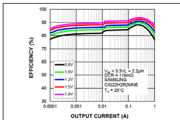
FIGURE 2-7: Buck Efficiency (LDCR = 116 mΩ) vs. Output Current.
