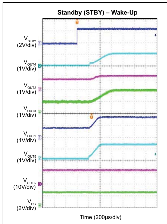
FIGURE 4-14: STBY-to-NORMAL Transition (DEFAULT).
