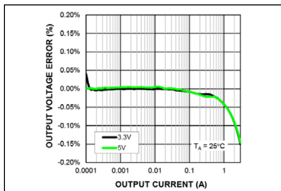
FIGURE 2-11: Buck Output Voltage Regulator vs. Output Current.
