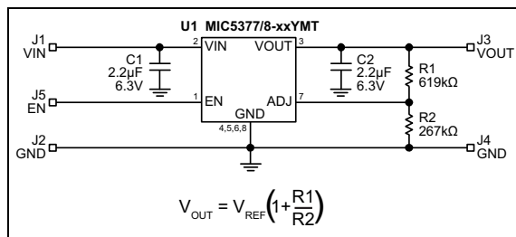
FIGURE 4-1: Adjustable Regulator with Resistors.
