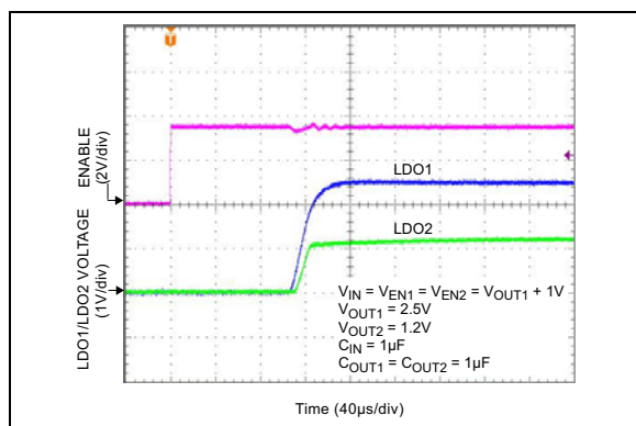
FIGURE 2-14: Enable Turn-On.
