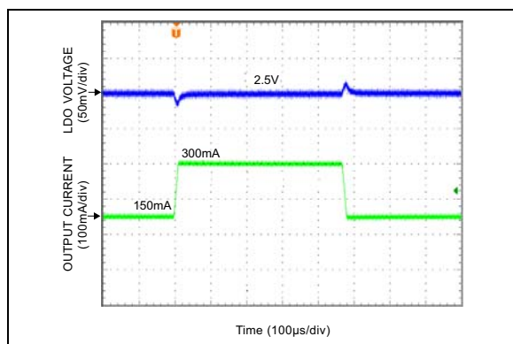
FIGURE 2-13: Load Transient (150 mA – 300 mA).
