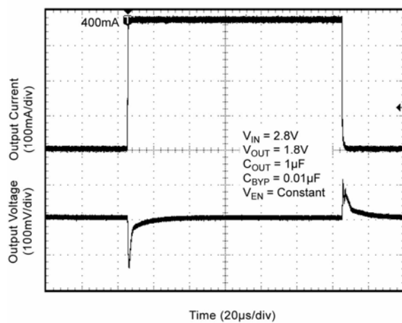
Load Transient ( V_{IN} )
