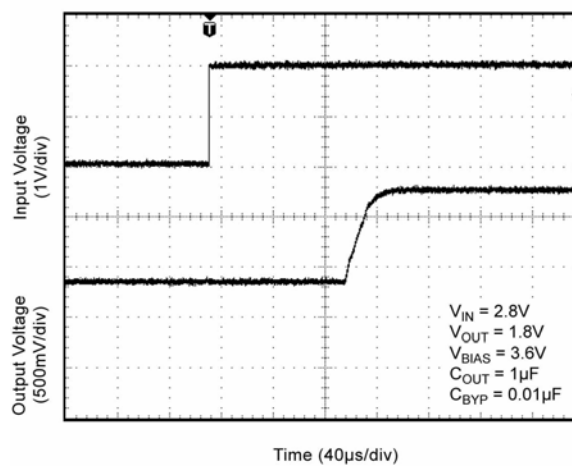
Turn-on Time
