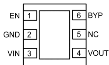
MIC5319-x.xBML/YML 6-Pin 2mm × 2mm MLF® (ML) Top View
