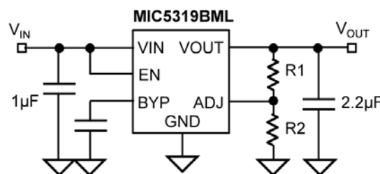
Figure 1. Adjustable Voltage Application
