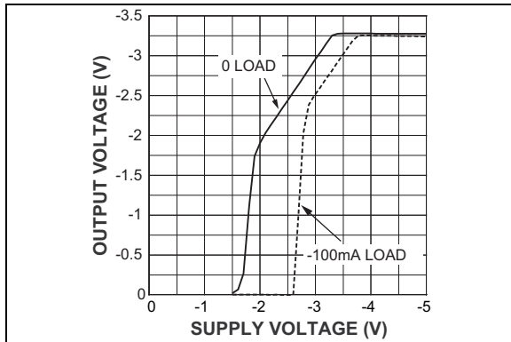
FIGURE 2-1: Dropout Characteristics.
