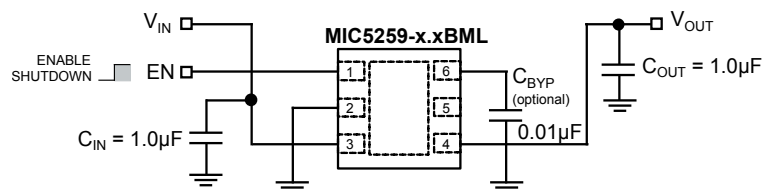
Ultra-Low-Noise Regulator Application
