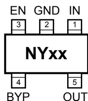
MIC5259-x.xBD5 ThinSOT™-23-5 (D5) (Top View)
