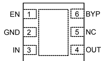
MIC5259-x.xBML 6-Pin 2mm × 2mm MLF™ (ML) (Top View)
