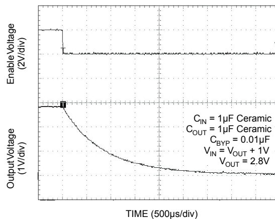
Enable Turn-Off
