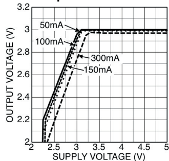
Dropout Characteristics
