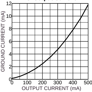
Ground Current vs. Output Current
