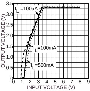
Dropout Characteristics
