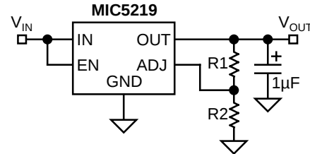
Figure 7. Low-Noise Adjustable Voltage Regulator
