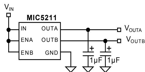
Figure 1. Thermal Conditions Circuit
