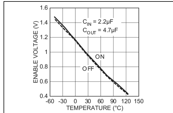
FIGURE 2-24: Enable Voltage Threshold vs. Temperature.
