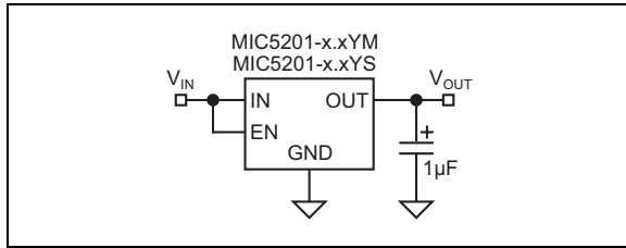
FIGURE 4-1: Fixed Application.
