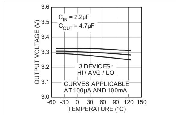
FIGURE 2-10: Output Voltage vs. Temperature (3.3V Version).
