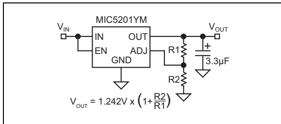
FIGURE 4-2: Adjustable Application.
