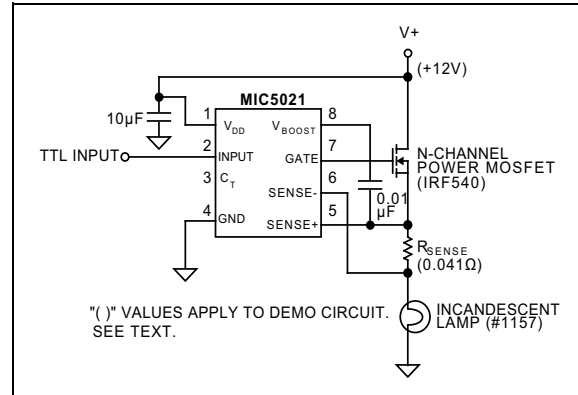
FIGURE 6-11: Lamp Driver with Current Sensing.
