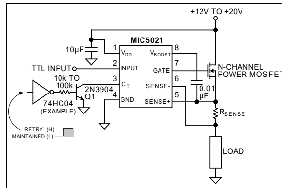
FIGURE 6-12: Remote Control Circuit.
