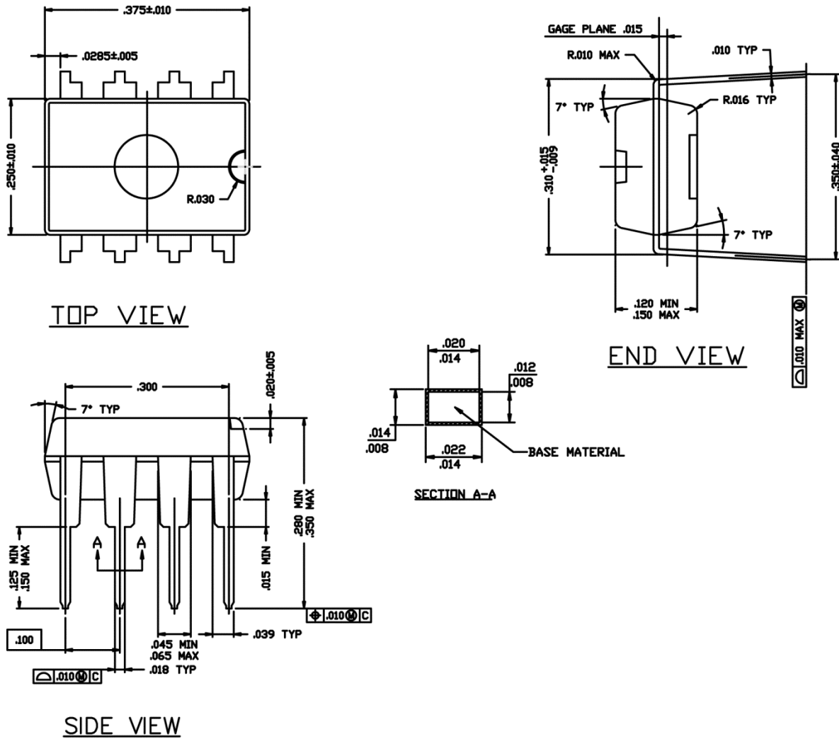
8-Pin Plastic DIP (N)
